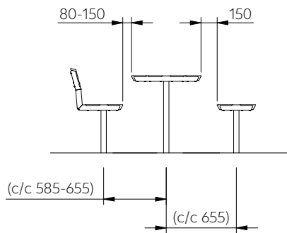
DAG500/501
