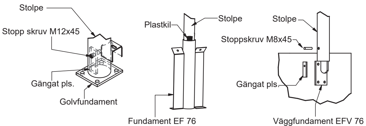
Figur 7. Fastbultning
